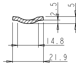
SECTION A-A SCALE 3:5
